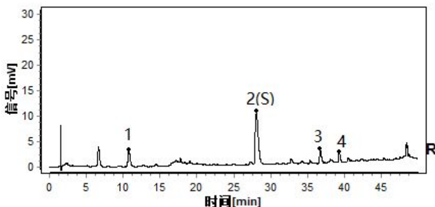
峰 2(S): 芥子碱硫氰酸盐 炒芥子(芥)配方颗粒对照特征图谱 色谱柱: CORTECS T3 C18; 2.1mm×150mm, 1.6μm
